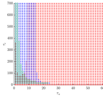
(b22) \rho = \phi = 0.4
