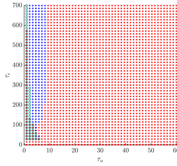
(b32) \rho = 0.7, \phi = 0.4
