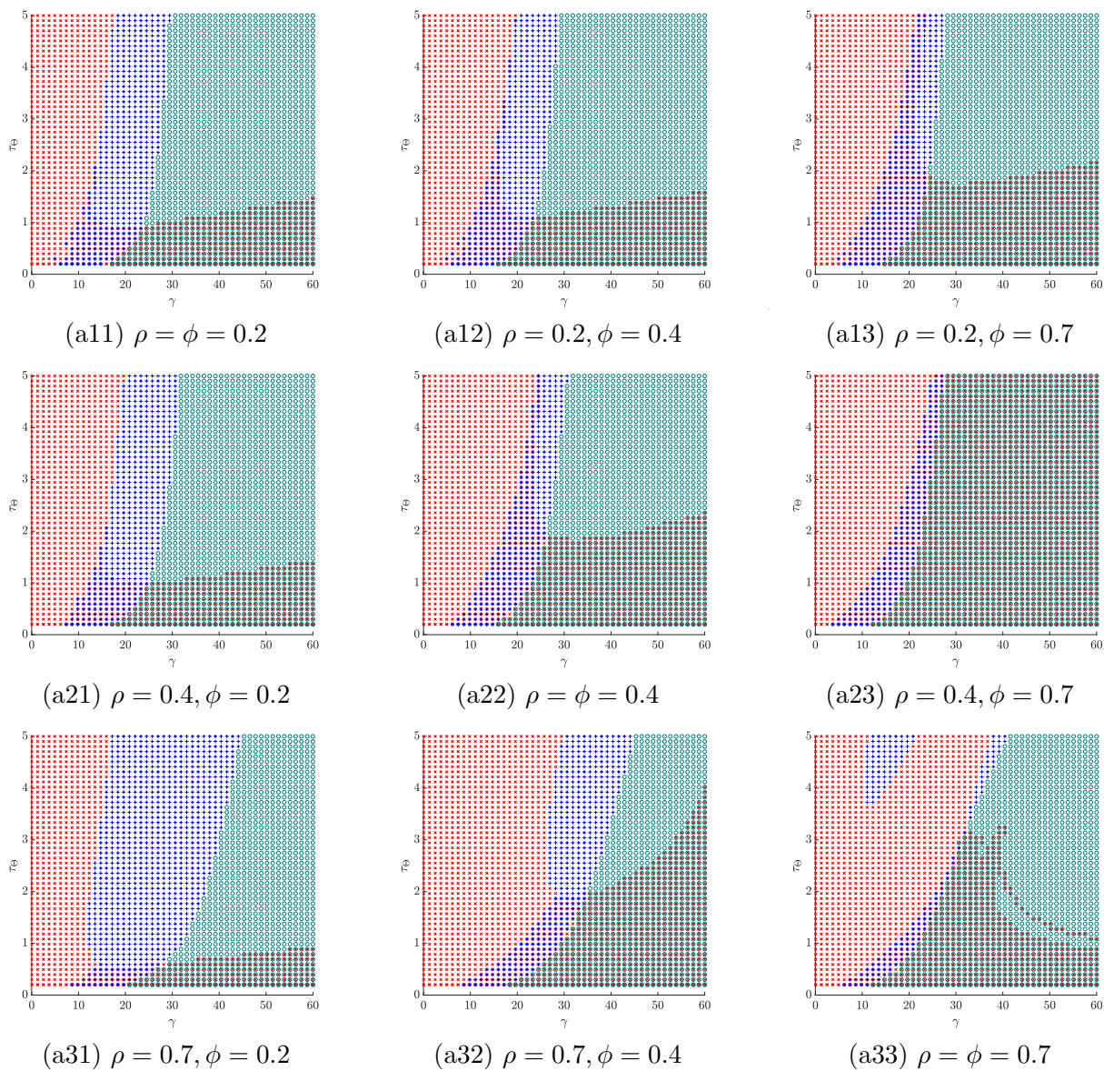
(a) Effect of \rho and \phi : (\gamma, \tau_\Theta)
