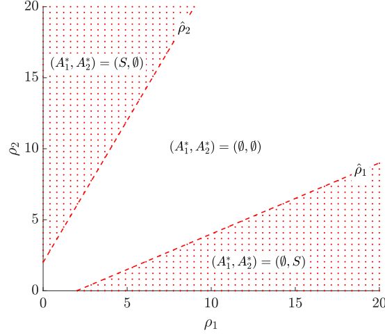
Figure 3: Information sharing between imperfectly informed investors
